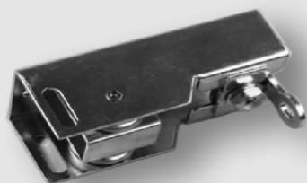
Single Draw Wheel 3071
